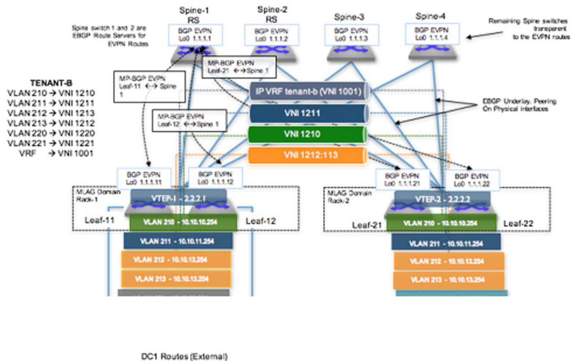
Figure 21-24: Tenant-B: Asymmetric IRB
