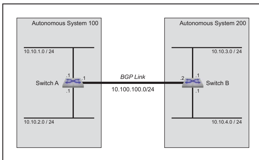
Figure 31-3: BGP Example 2
