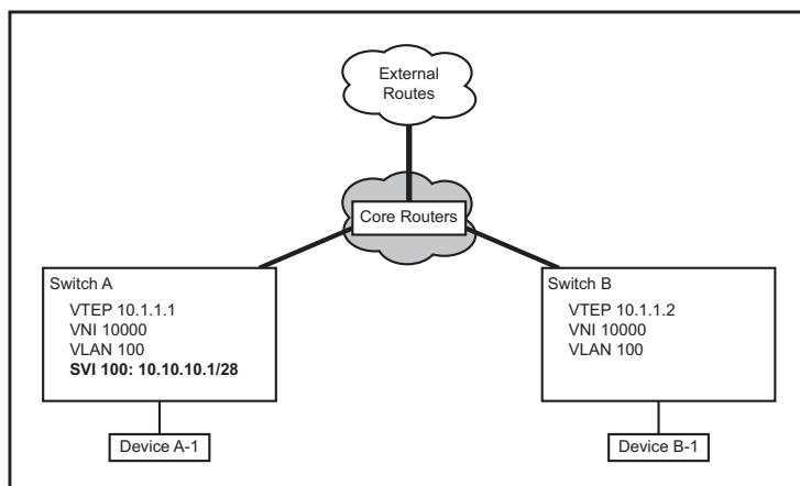
Figure 20-3: Implementing VXLAN Routing
