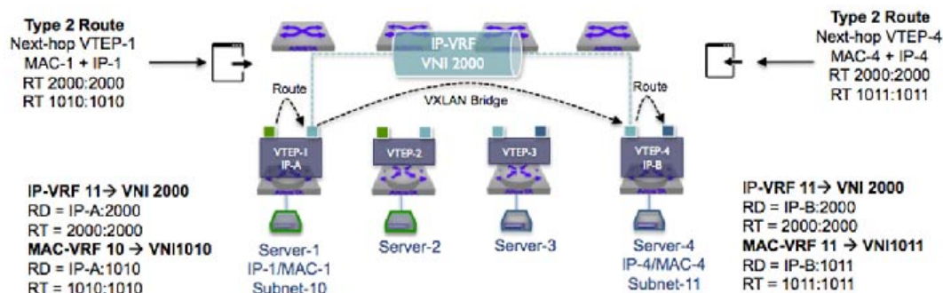
Figure 21-16: EVPN Symmetric IRB
