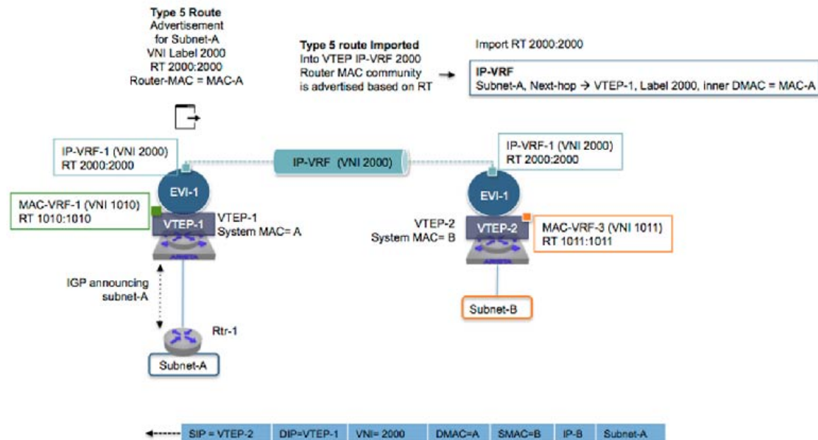
Figure 21-20: EVPN Route Type-5, Interface-less Update
