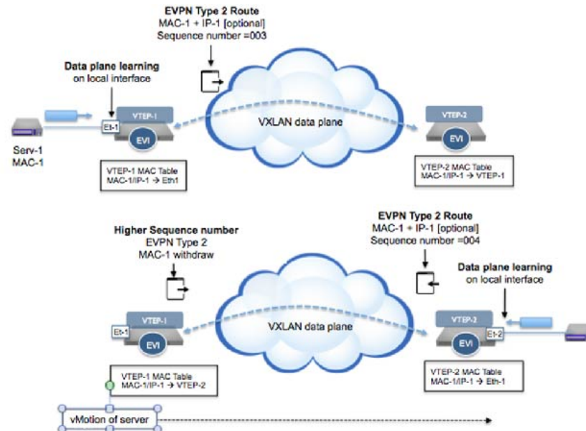
Figure 21-10: EVPN type-2 MAC Mobility Behavior
