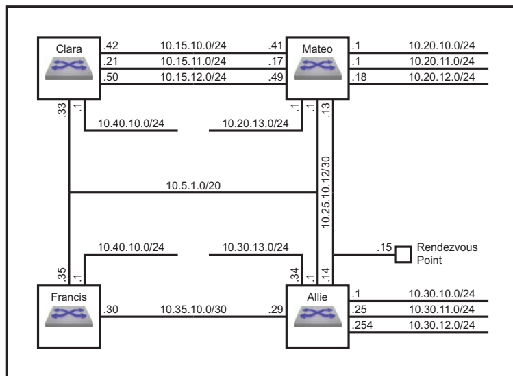
Figure 38-1: Multicast Example
