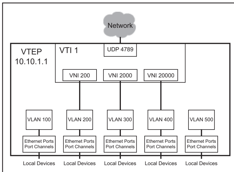
Figure 20-1: VXLAN Architecture
