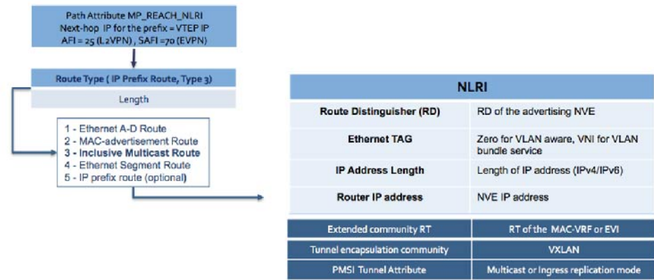
Figure 21-12: EVPN type-3 IMET Route Format
