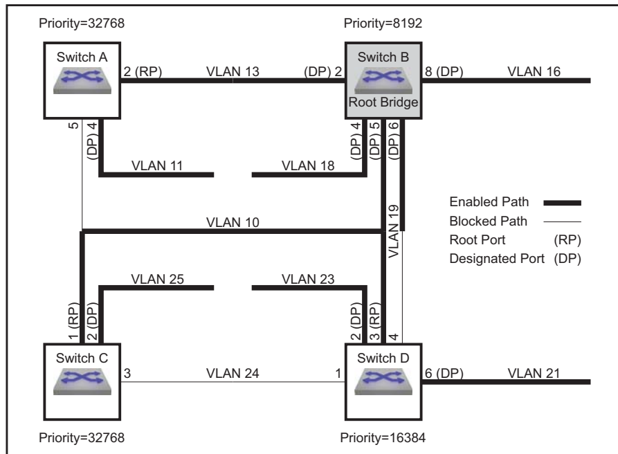
Figure 24-1: Spanning Tree Network Example
