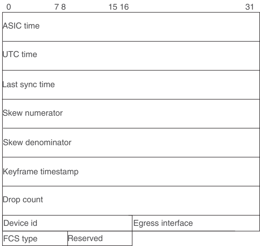
Figure 18-1: Key frame payload
