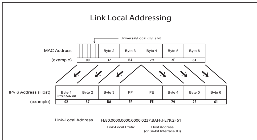
Figure 27-1: Link Local Address Derivation
