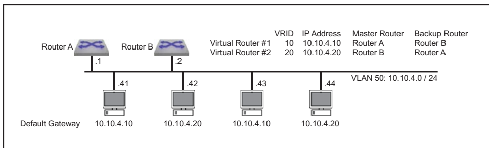
Figure 23-3: VRRP Example 2 Network Diagram
