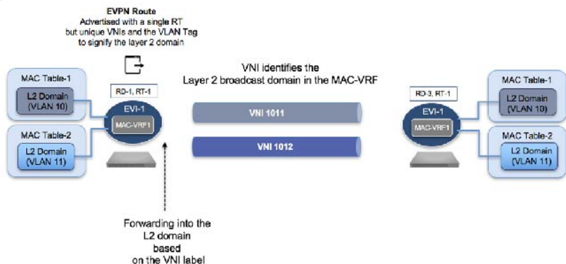
Figure 21-7: VLAN Aware Bundle Service
