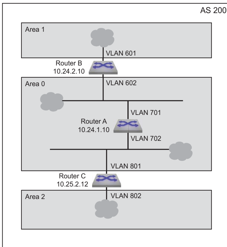
Figure 30-4: OSPFv3 Example 2
