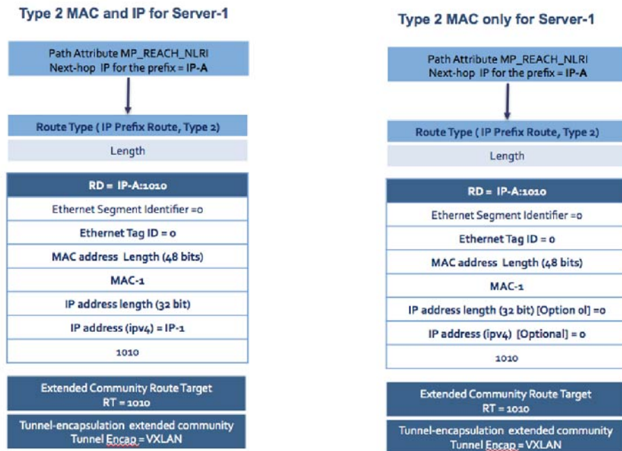
Figure 21-14: EVPN Comparison of MAC & MAC+IP Type 2 Route in Asymmetric IRB
