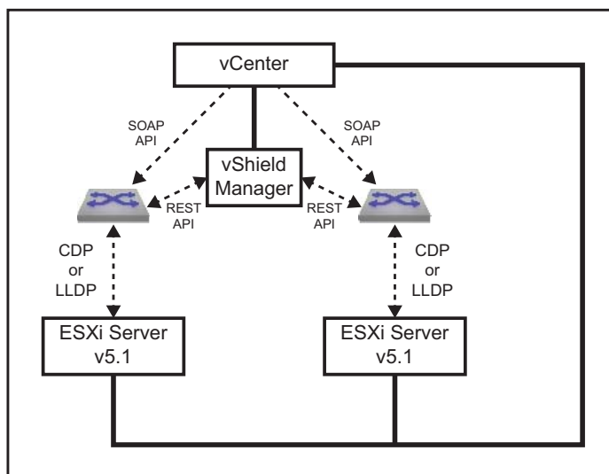
Figure 43-2: VM Tracer Topology – Monitoring VXLAN Based Configurations
