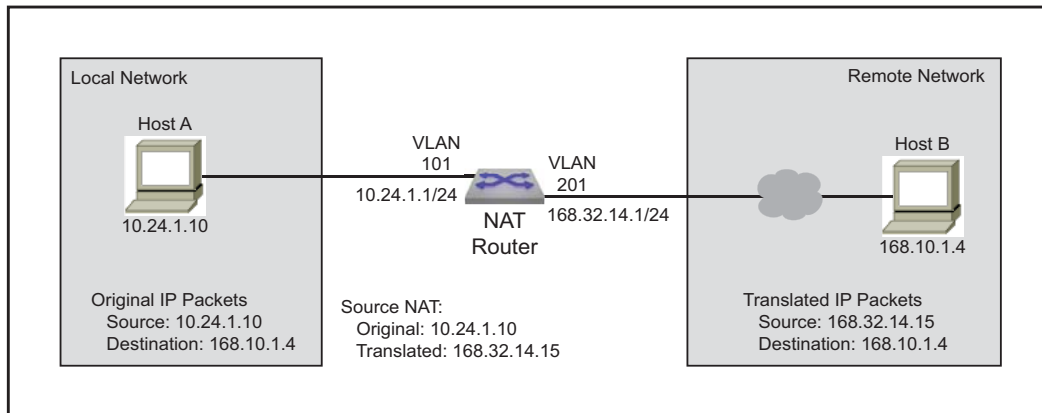
Figure 26-4: Source NAT Example
