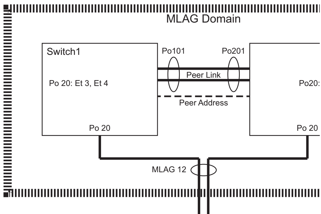
Figure 12-2: MLAG Interface Configuration
