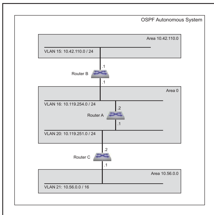
Figure 29-4: OSPFv2 Example 2
