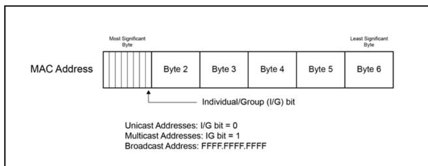
Figure 17-1: MAC Address Format
