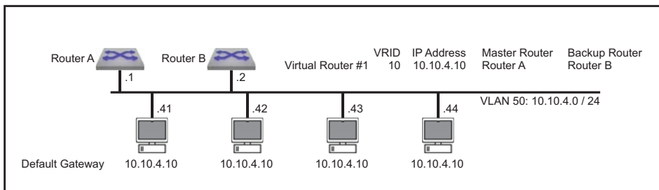
Figure 23-2: VRRP Example 1 Network Diagram
