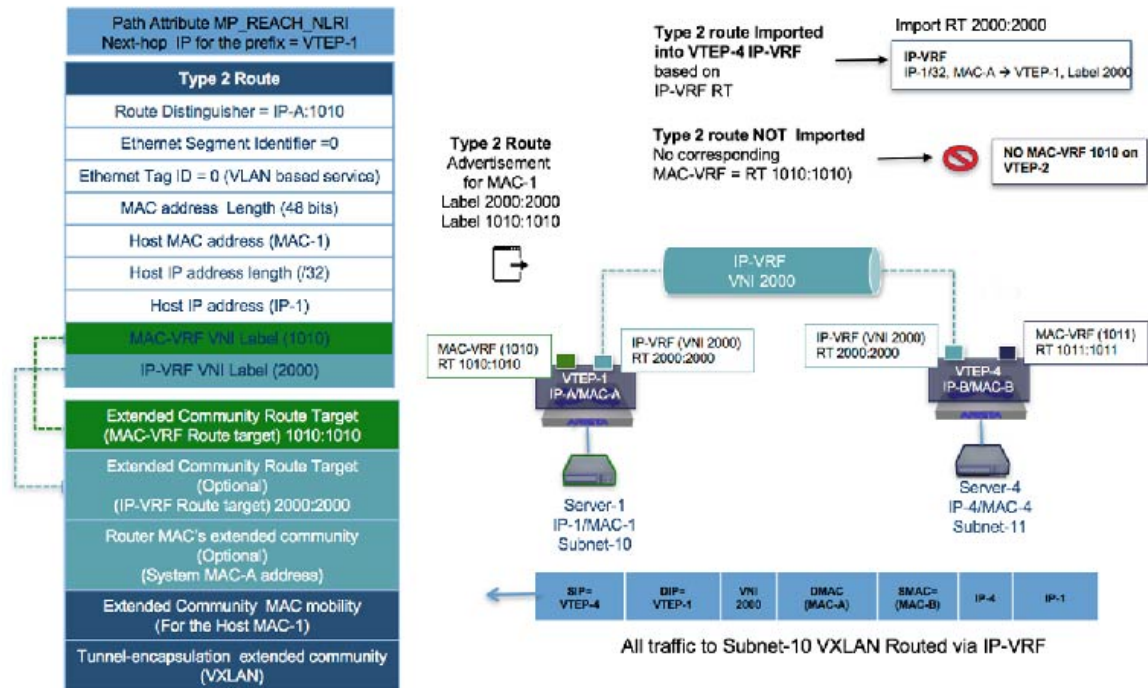
Figure 21-18: EVPN Type 2 Route in Symmetric IRB - MAC-VRF Only Exists on Sending VTEP
