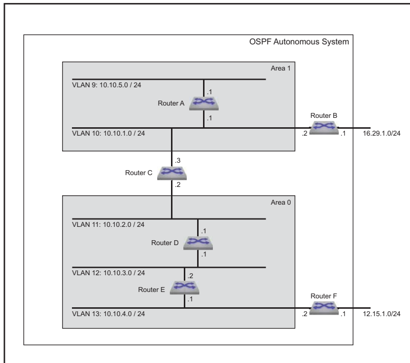
Figure 29-5: OSPFv2 Example 3
