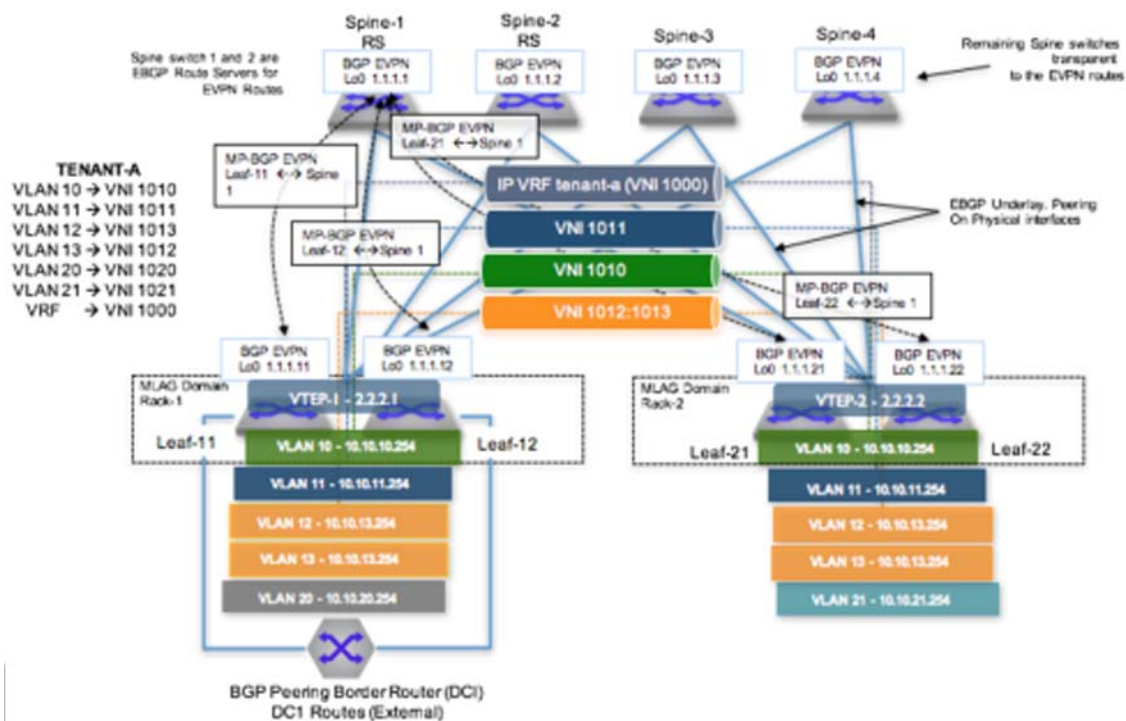
Figure 21-23: Tenant-A: Symmetric IRB
