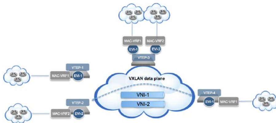
Figure 21-3: EVPN Terminology for a VXLAN Data Plane
