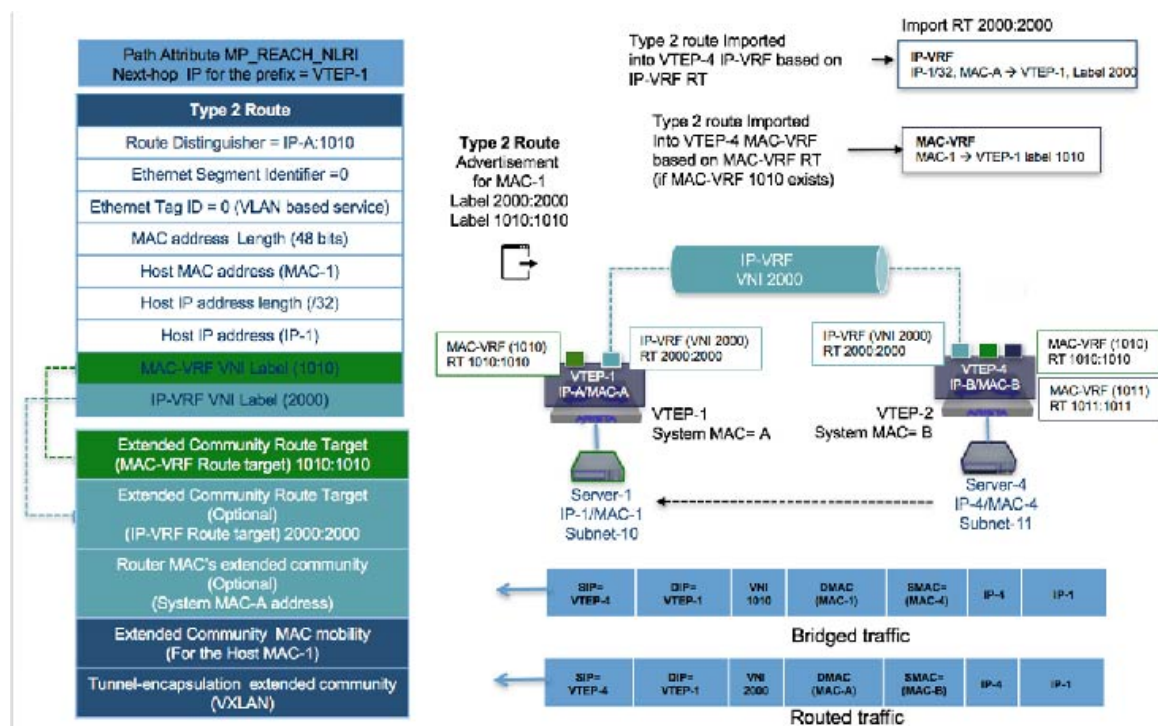
Figure 21-17: EVPN Type 2 Route in Symmetric IRB - MAC-VRF on Both VTEPs
