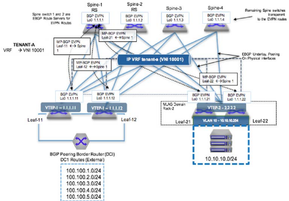
Figure 21-22: Layer 3 EVPN Configuration
