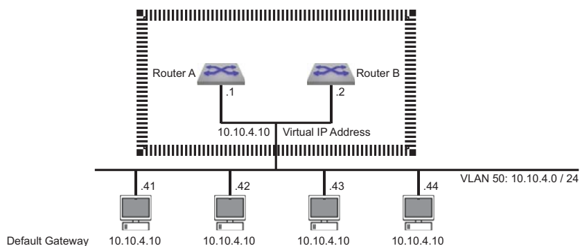
Figure 23-1: VARP Configuration
