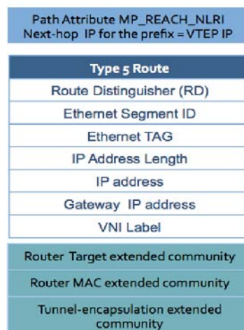
Figure 21-19: EVPN Route Type-5, for Advertisement of IP Prefixes
