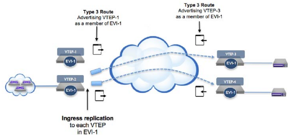
Figure 21-11: EVPN type-3 IMET Route Behavior for Ingress Replication
