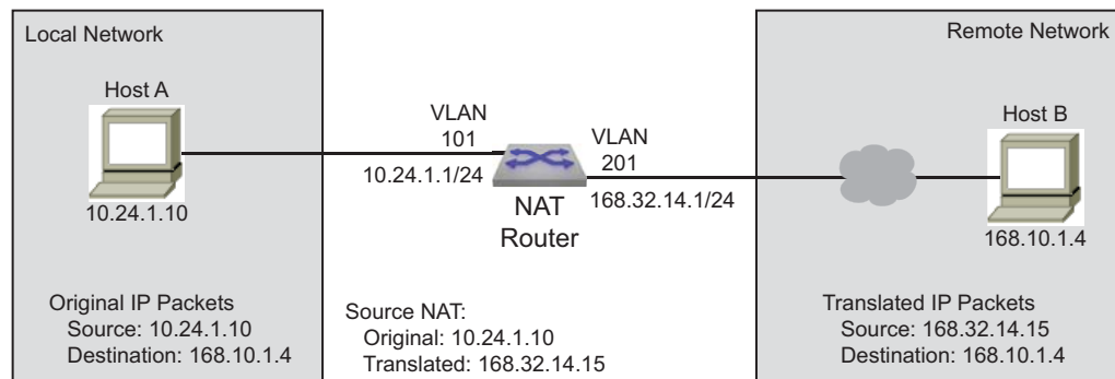
Figure 26-5: Destination NAT Example
