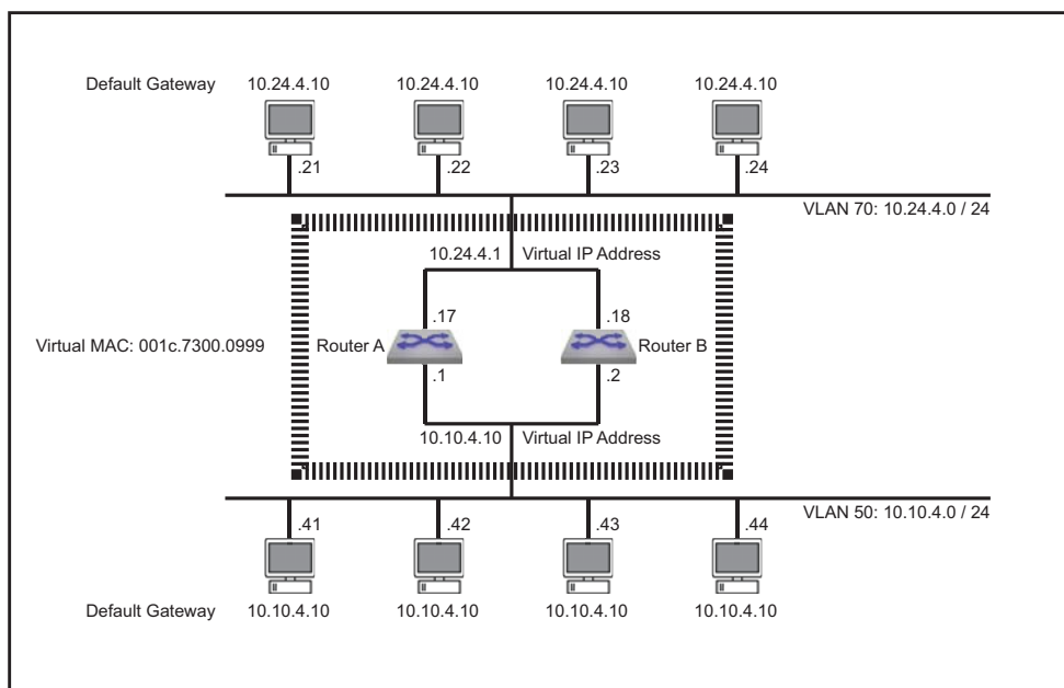
Figure 23-5: VARP Example Network Diagram
