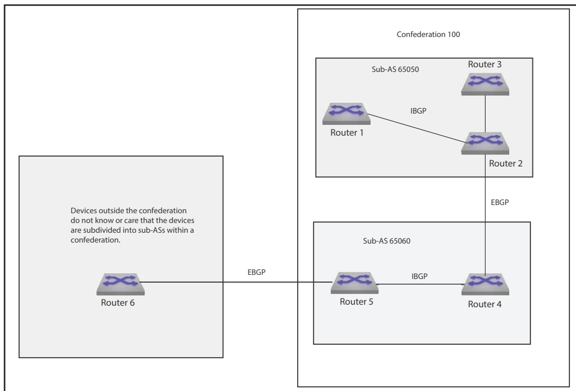
Figure 31-1: BGP Confederation Example
