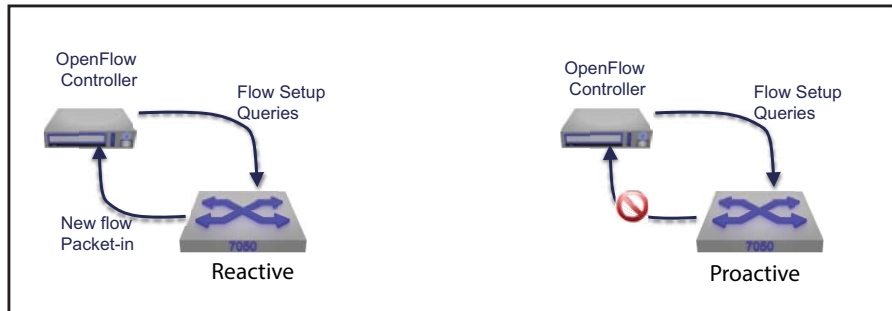
Figure 47-1: Reactive and proactive modes
