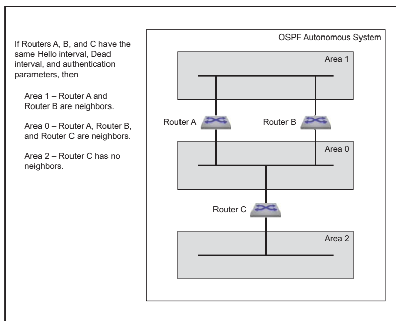
Figure 29-2: OSPFv2 Neighbors
