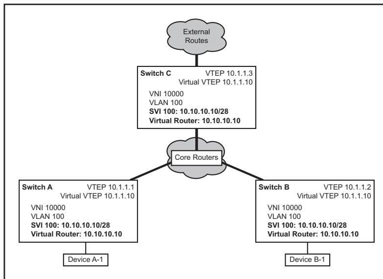
Figure 20-4: Direct VXLAN Routing
