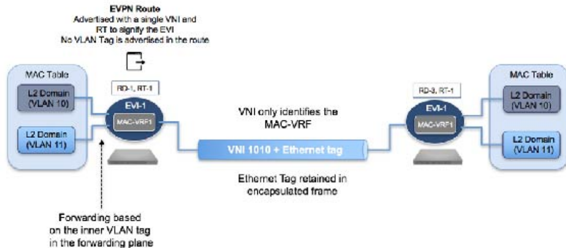
Figure 21-6: VLAN Bundle Service Interface
