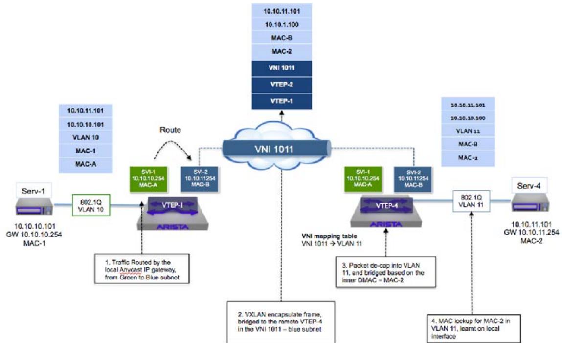
Figure 21-15: EVPN Asymmetric IRB VxLAN Data-plane Forwarding Detail
