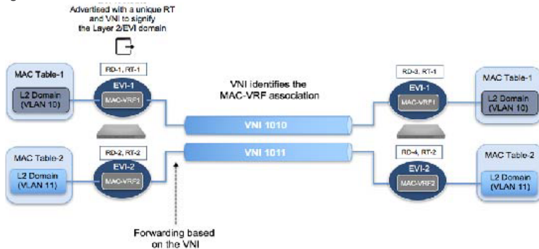
Figure 21-5: VLAN Based Service Interface
