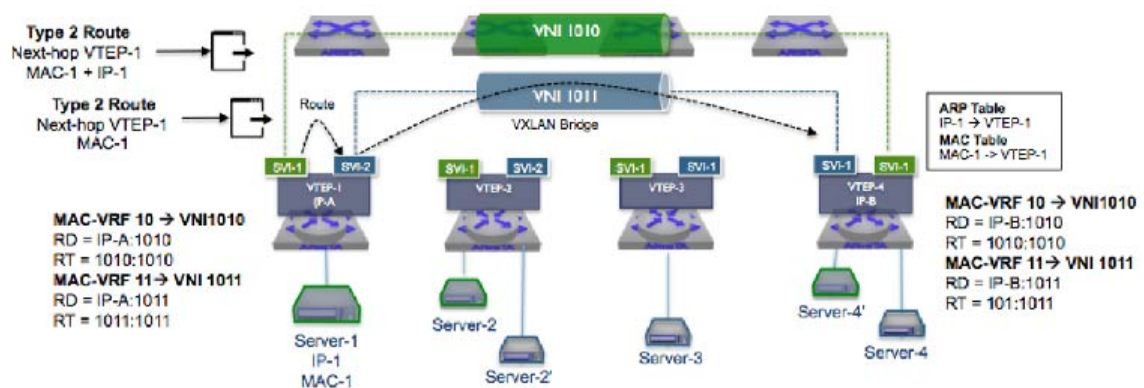
Figure 21-13: EVPN Asymmetric IRB
