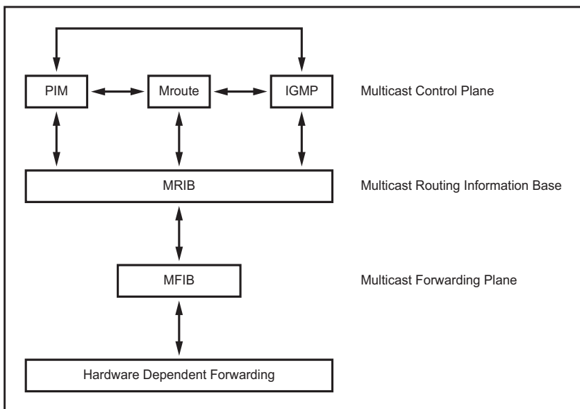
Figure 36-1: Multicast Architecture
