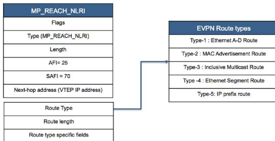
Figure 21-4: EVPN NLRI Route Format
