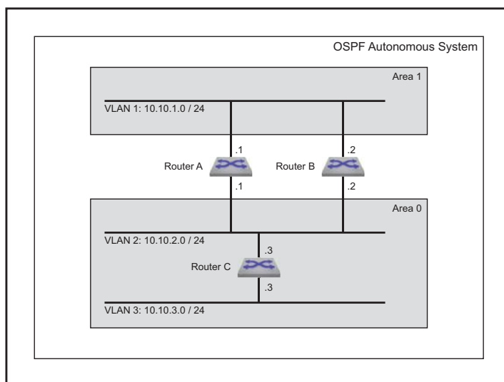
Figure 29-3: OSPFv2 Example 1
