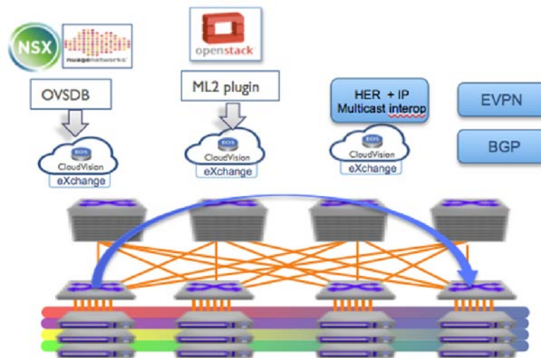
Figure 21-1: Different VXLAN Control Planes
