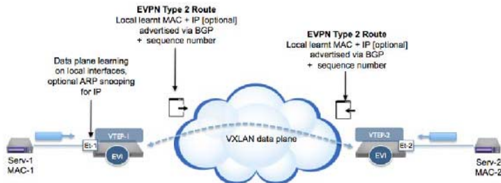
Figure 21-8: EVPN Type 2 Route Announcement
