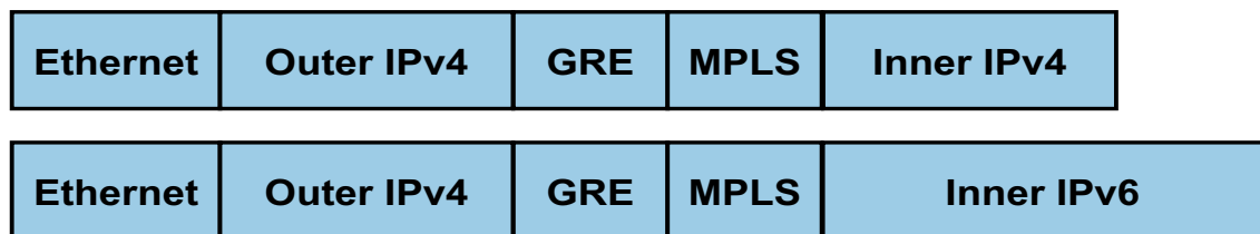
Figure 34-1: Header Format of Packets
