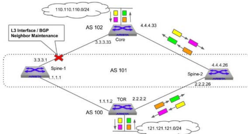
Figure 9-2: Traffic flow pattern between TOR and Core – After unit on Spine-1 is put into Maintenance
